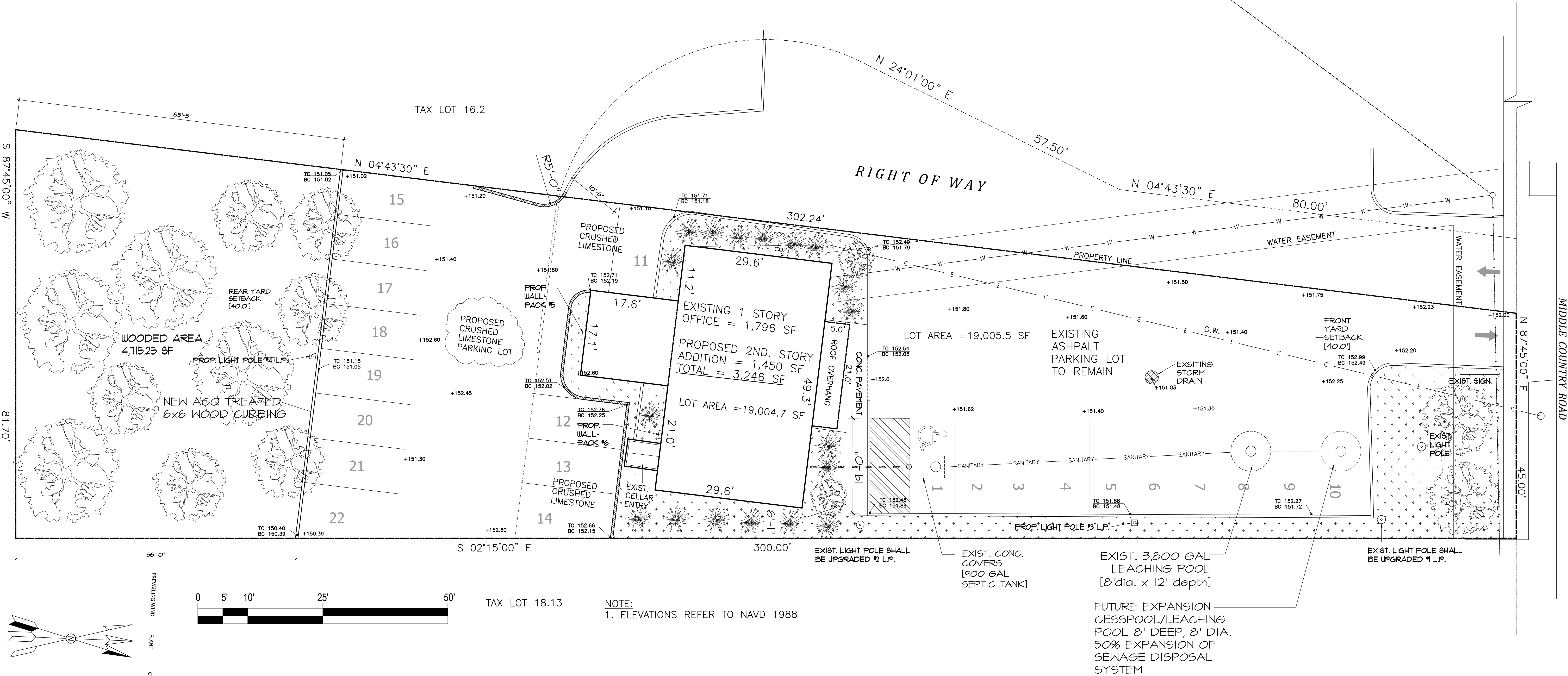
PROPOSED & EXISTING GRADING PLAN SCALE: 1/16" = 1'-0"
